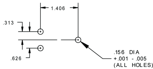
MOUNTING DIMENSIONS
