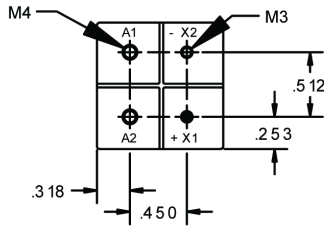
TERMINAL LAYOUT
