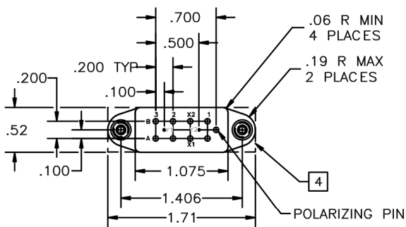
SOCKET DRAWING
